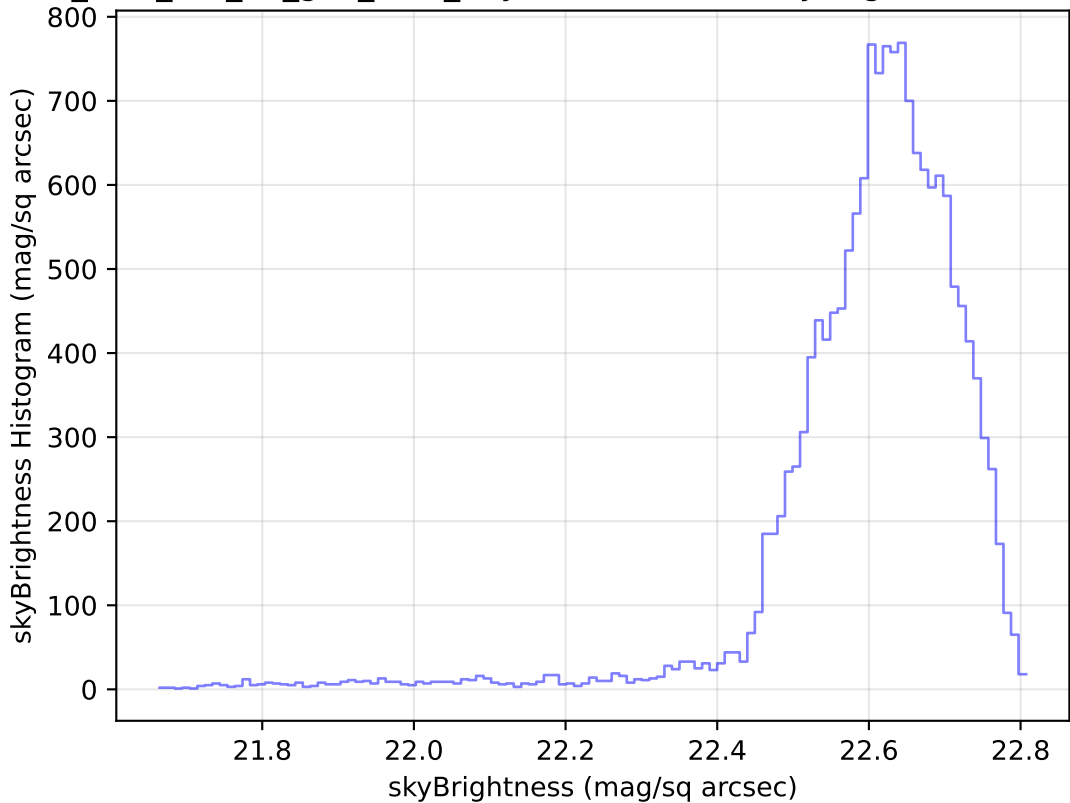
too_elab_r16_d3_griz_v3.4_10yrs Yr 1 u band: skyBrightness Histogram
