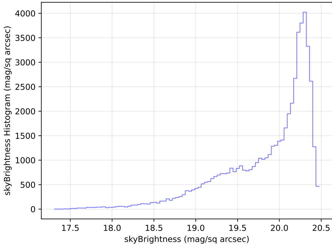
too_elab_r16_d3_griz_v3.4_10yrs Yr 1 i band: skyBrightness Histogram
