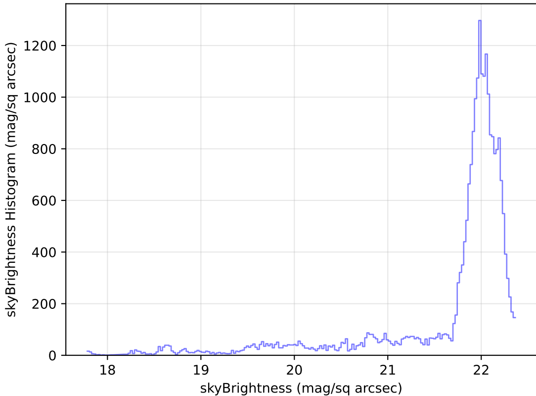
too_elab_r16_d3_griz_v3.4_10yrs Yr 1 g band: skyBrightness Histogram
