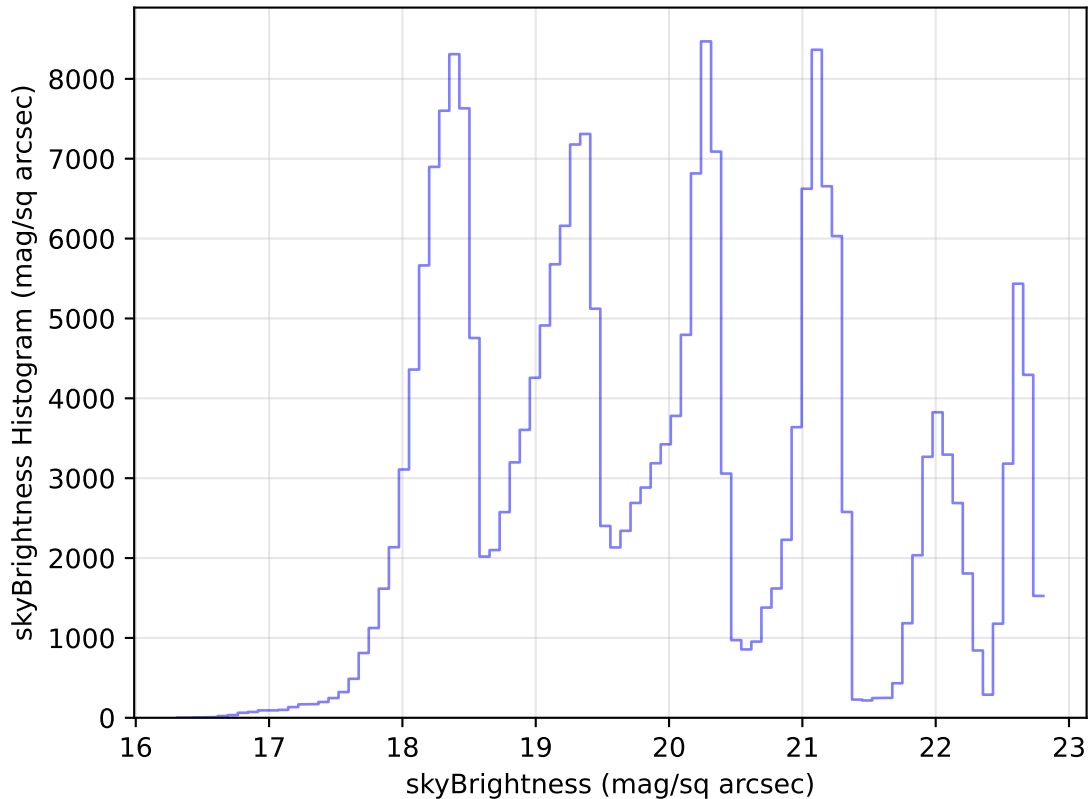
too_elab_r16_d3_griz_v3.4_10yrs Yr 1 all bands: skyBrightness Histogram
