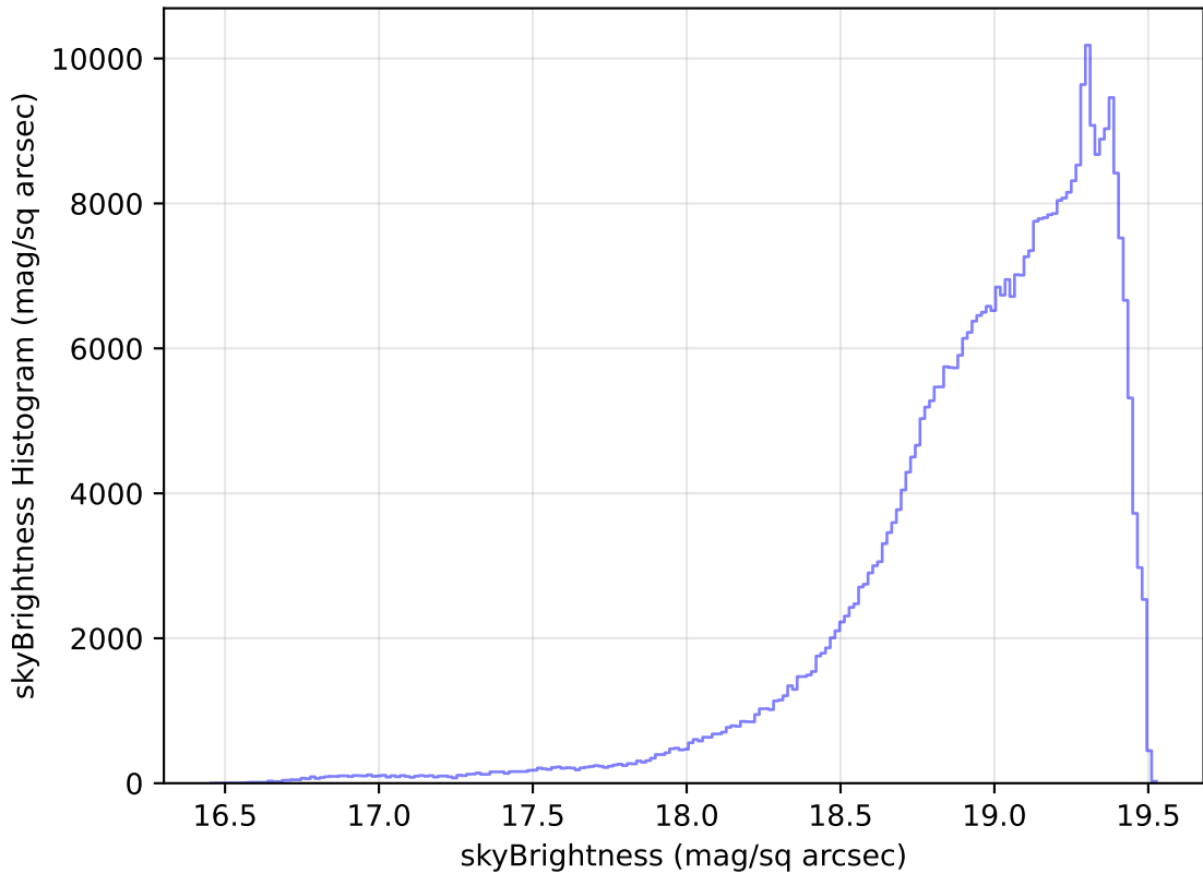
too_elab_r16_d3_griz_v3.4_10yrs WFD z band: skyBrightness Histogram
