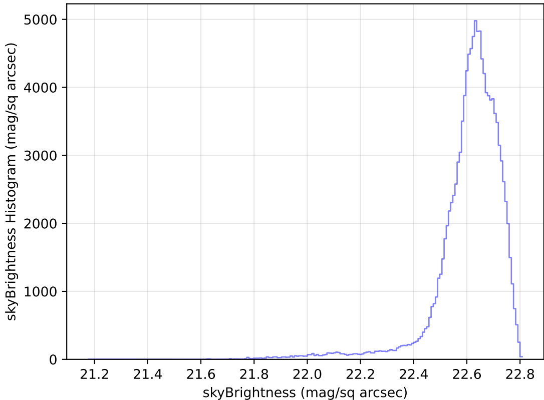
too_elab_r16_d3_griz_v3.4_10yrs WFD u band: skyBrightness Histogram
