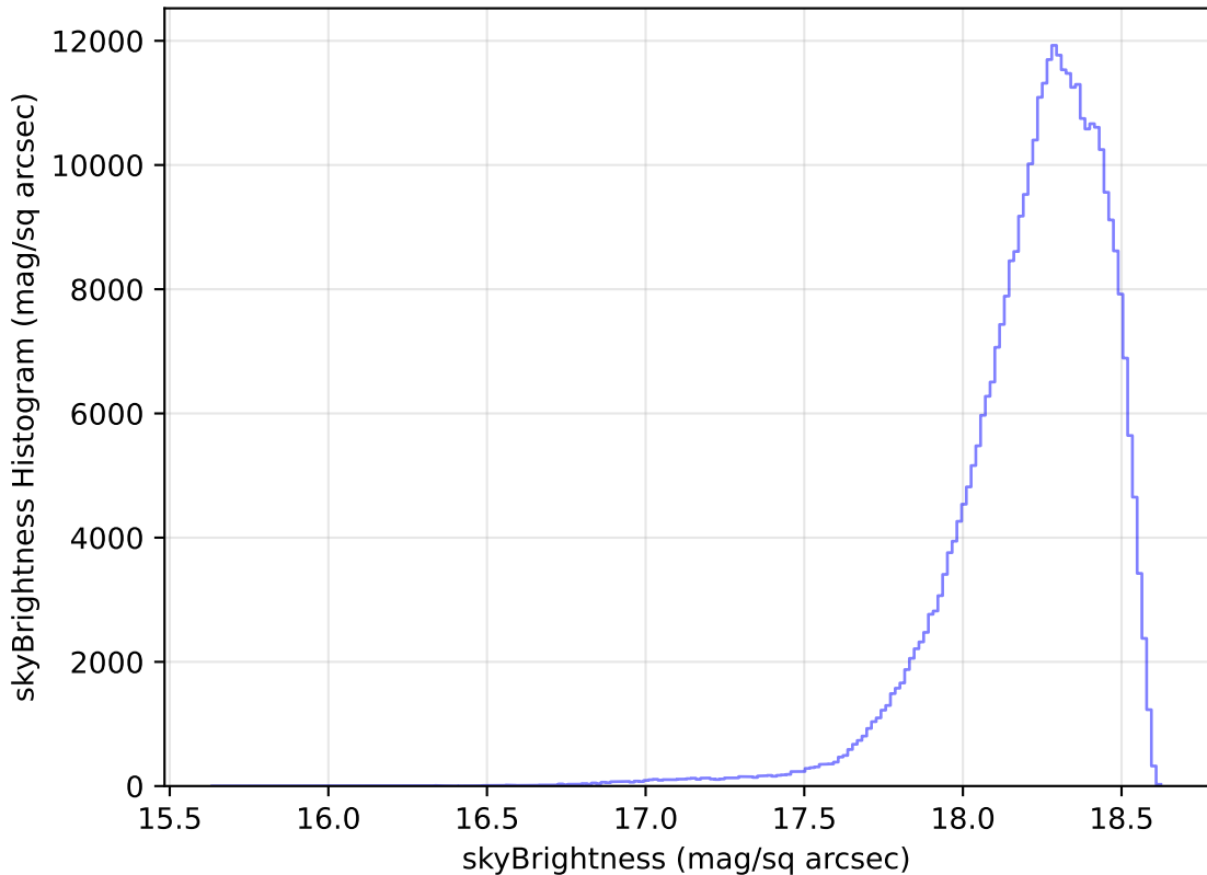
too_elab_r16_d3_griz_v3.4_10yrs All sky y band: skyBrightness Histogram
