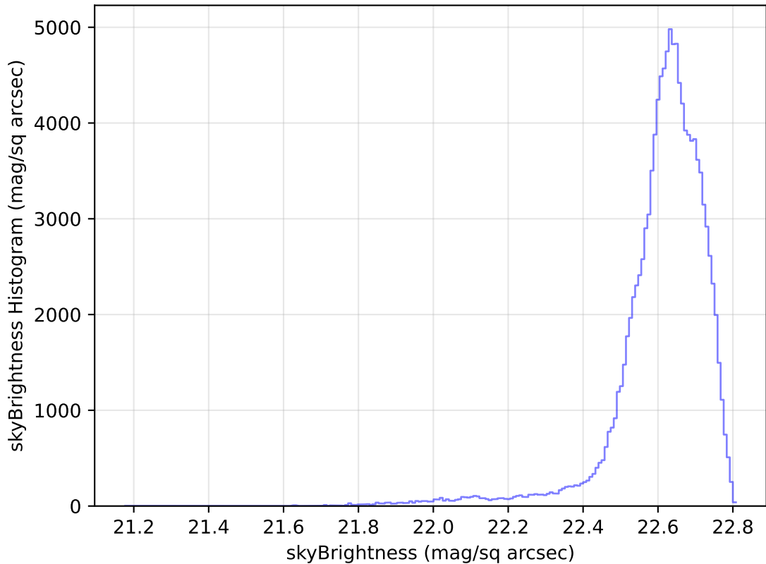
too_elab_r16_d3_griz_v3.4_10yrs All sky u band: skyBrightness Histogram
