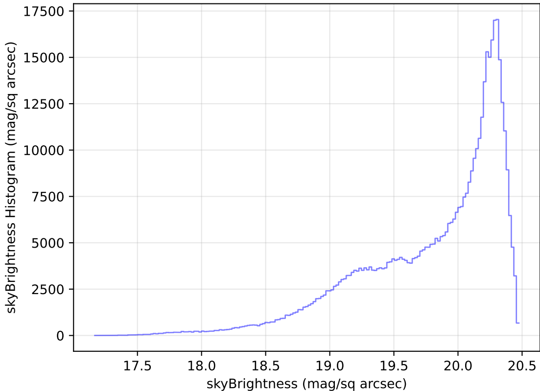
too_elab_r16_d3_griz_v3.4_10yrs All sky i band: skyBrightness Histogram
