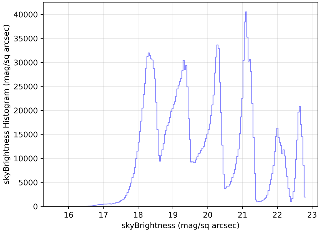
too_elab_r16_d3_griz_v3.4_10yrs All sky all bands: skyBrightness Histogram
