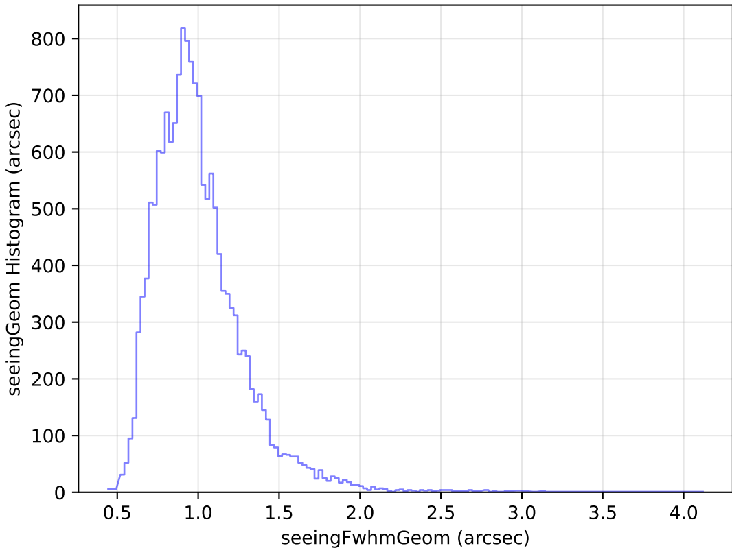
too_elab_r16_d3_griz_v3.4_10yrs Yr 1 u band: seeingGeom Histogram
