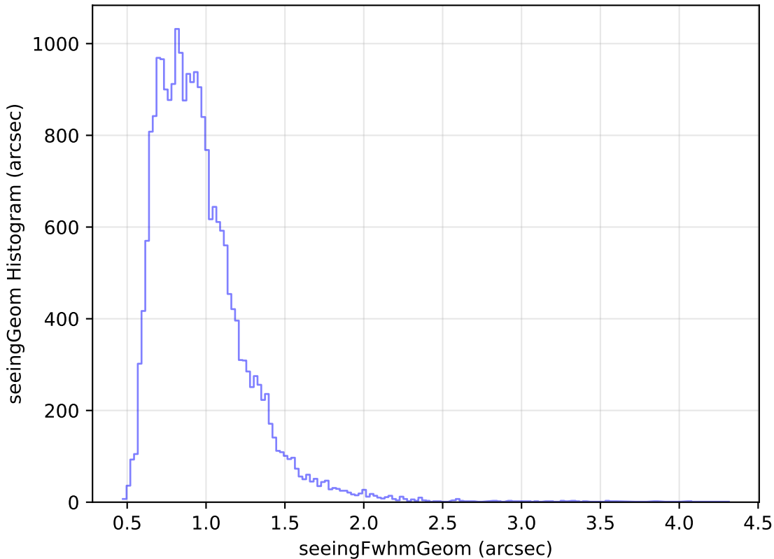
too_elab_r16_d3_griz_v3.4_10yrs Yr 1 g band: seeingGeom Histogram
