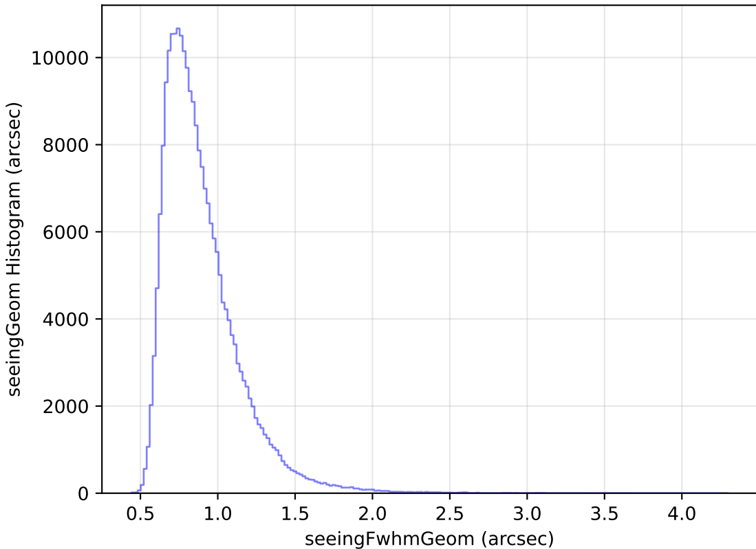
too_elab_r16_d3_griz_v3.4_10yrs Yr 1 all bands: seeingGeom Histogram
