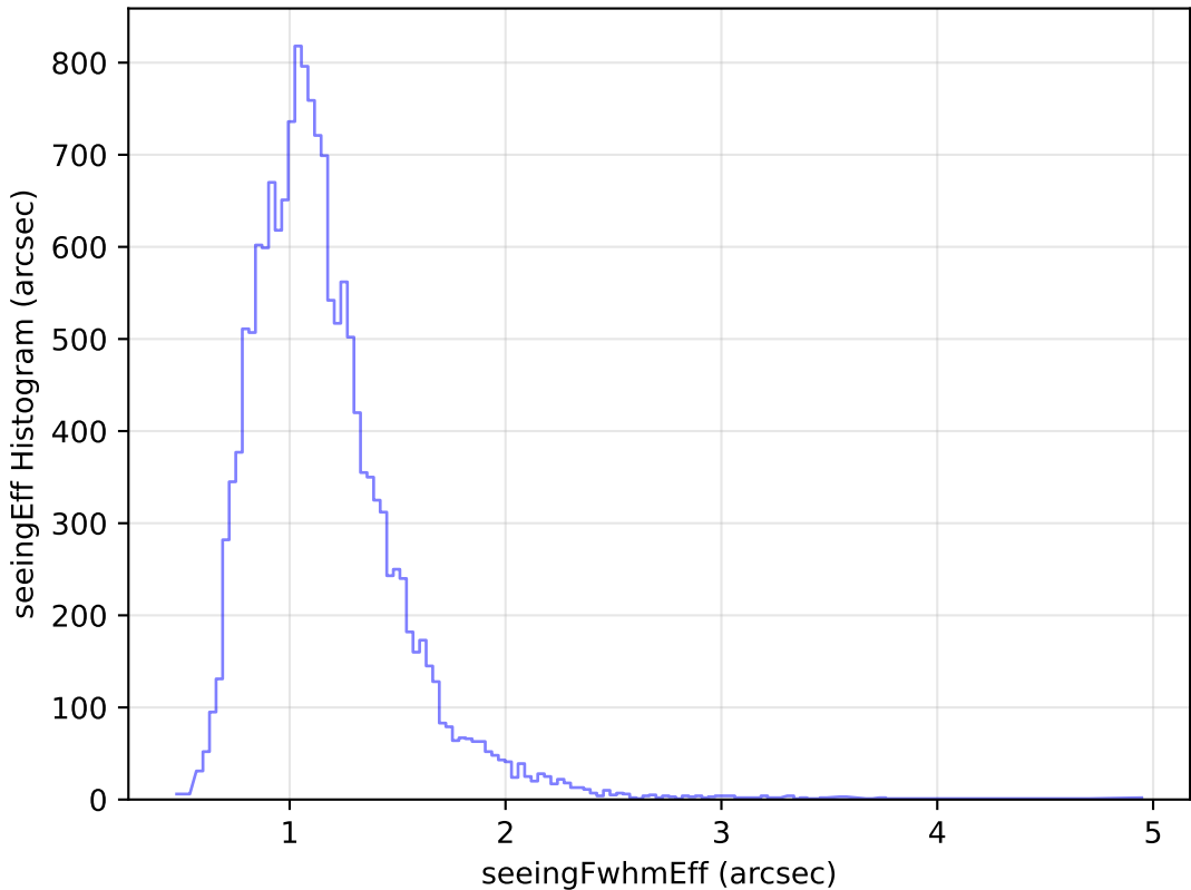
too_elab_r16_d3_griz_v3.4_10yrs Yr 1 u band: seeingEff Histogram
