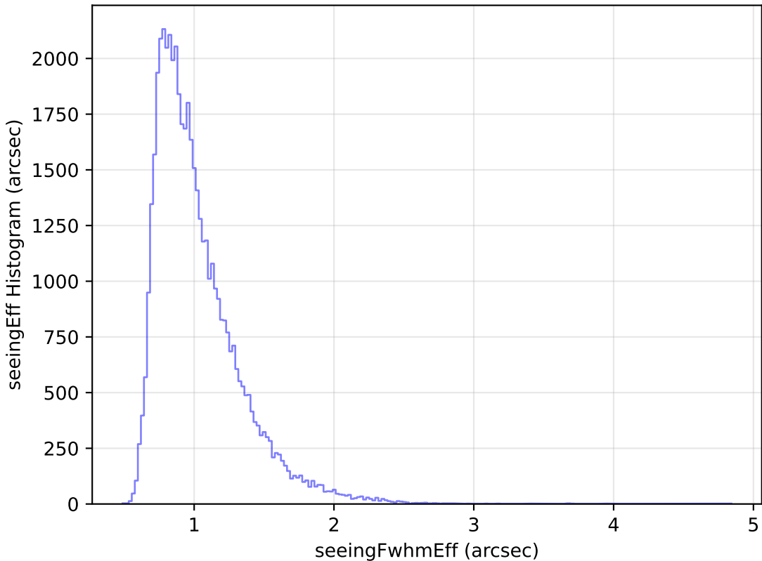
too_elab_r16_d3_griz_v3.4_10yrs Yr 1 r band: seeingEff Histogram
