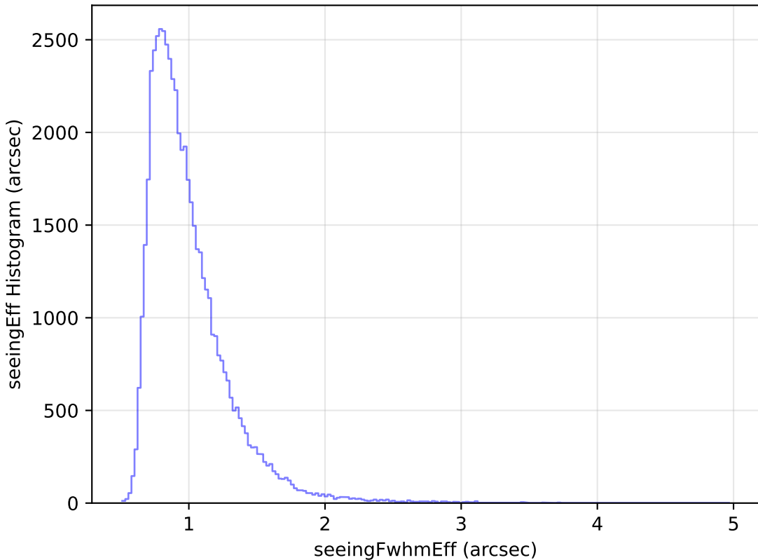
too_elab_r16_d3_griz_v3.4_10yrs Yr 1 i band: seeingEff Histogram
