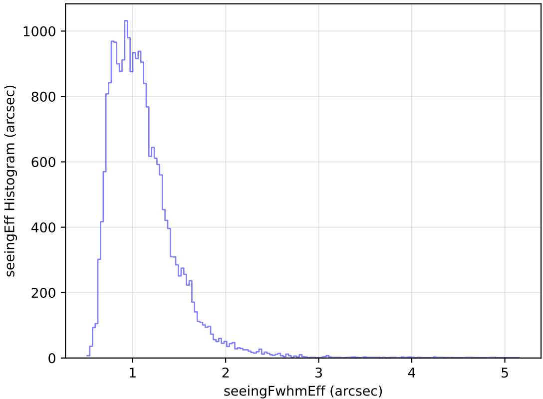
too_elab_r16_d3_griz_v3.4_10yrs Yr 1 g band: seeingEff Histogram
