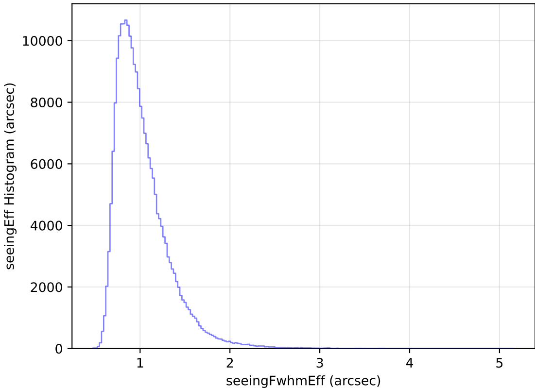
too_elab_r16_d3_griz_v3.4_10yrs Yr 1 all bands: seeingEff Histogram
