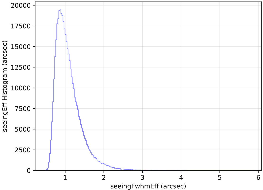
too_elab_r16_d3_griz_v3.4_10yrs WFD z band: seeingEff Histogram
