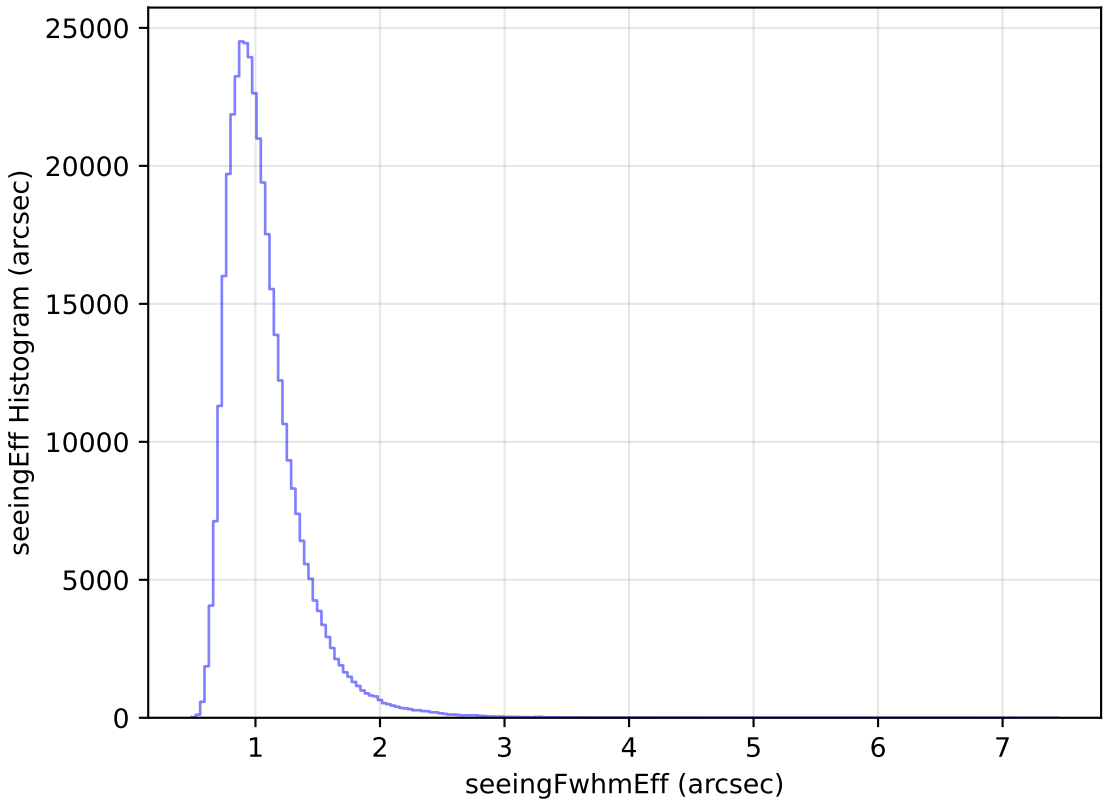
too_elab_r16_d3_griz_v3.4_10yrs WFD y band: seeingEff Histogram
