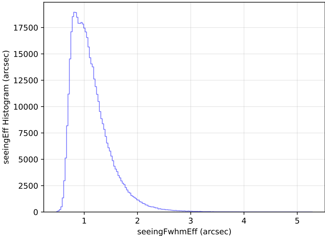
too_elab_r16_d3_griz_v3.4_10yrs WFD r band: seeingEff Histogram
