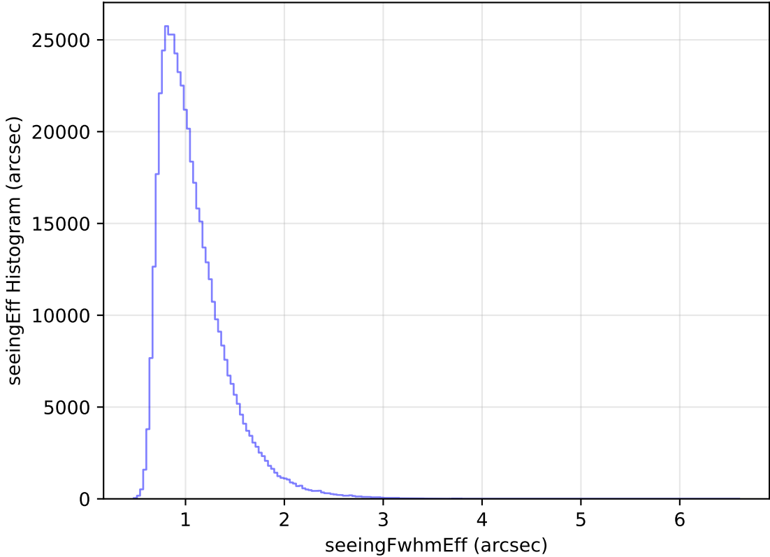
too_elab_r16_d3_griz_v3.4_10yrs WFD i band: seeingEff Histogram
