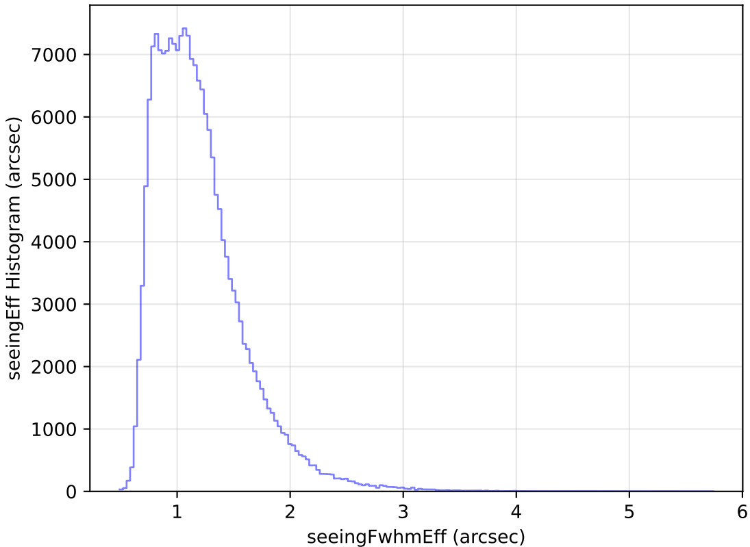
too_elab_r16_d3_griz_v3.4_10yrs WFD g band: seeingEff Histogram
