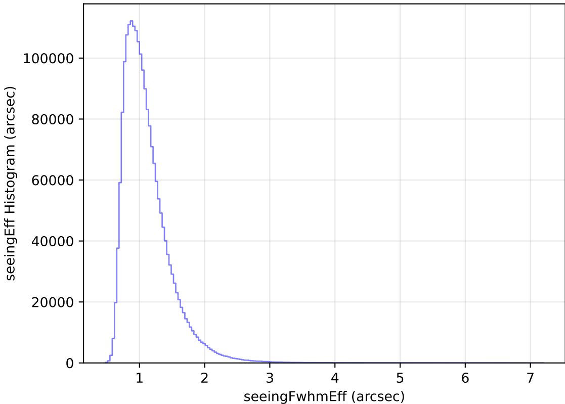
too_elab_r16_d3_griz_v3.4_10yrs WFD all bands: seeingEff Histogram
