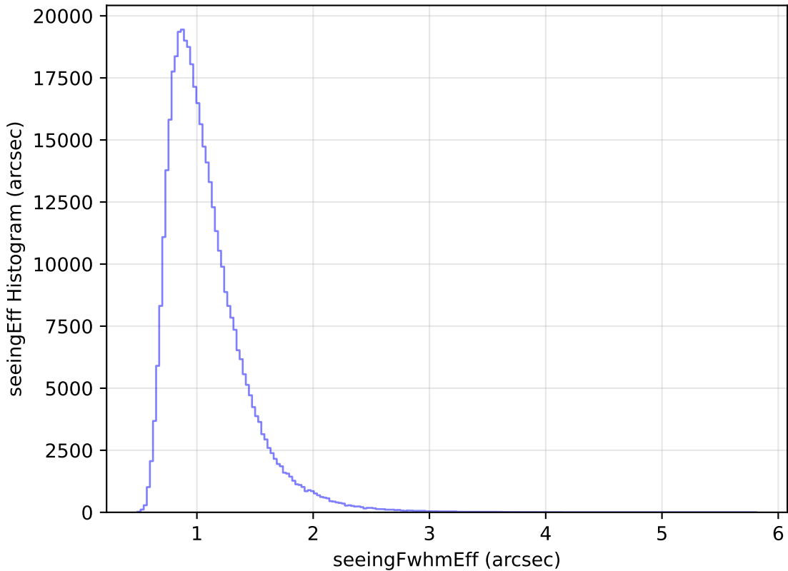
too_elab_r16_d3_griz_v3.4_10yrs All sky z band: seeingEff Histogram
