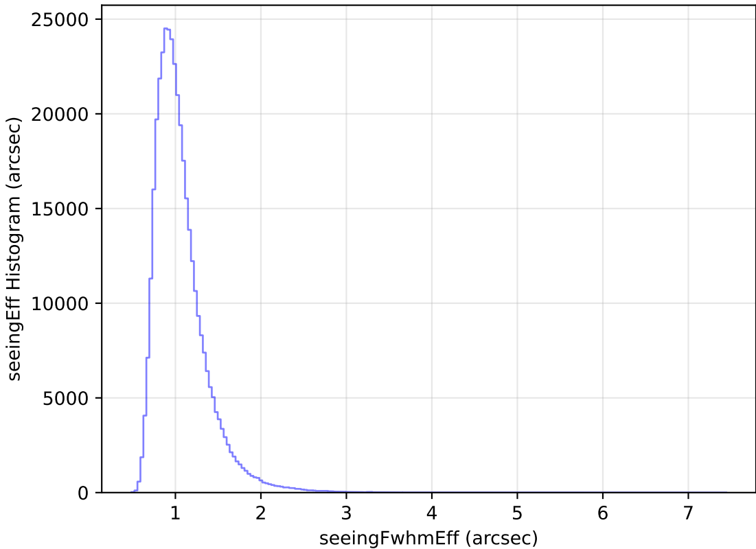
too_elab_r16_d3_griz_v3.4_10yrs All sky y band: seeingEff Histogram
