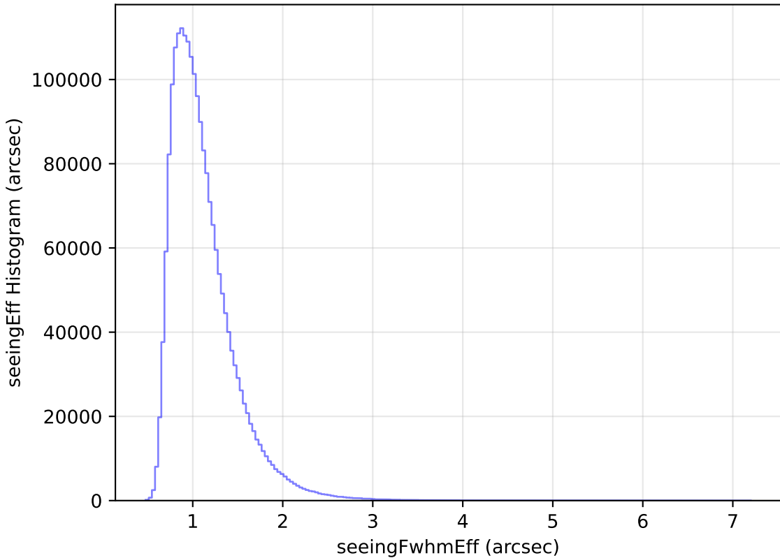
too_elab_r16_d3_griz_v3.4_10yrs All sky all bands: seeingEff Histogram
