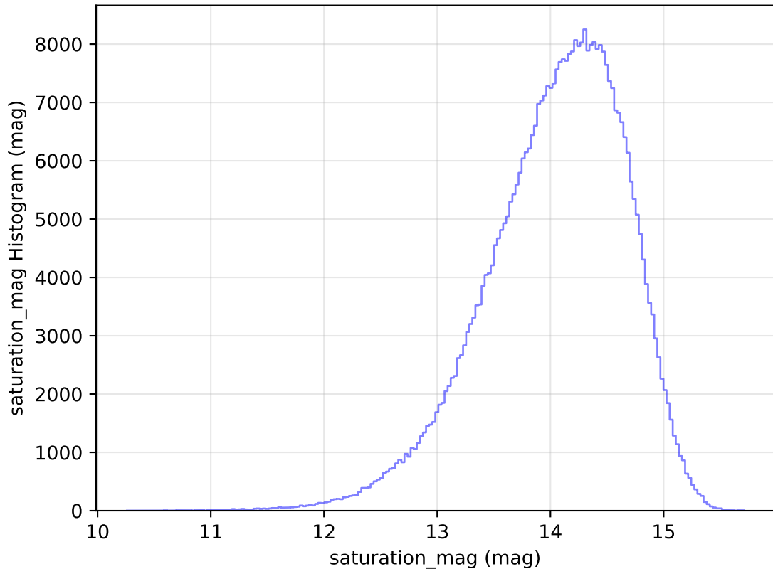
too_elab_r16_d3_griz_v3.4_10yrs WFD z band: saturation_mag Histogram
