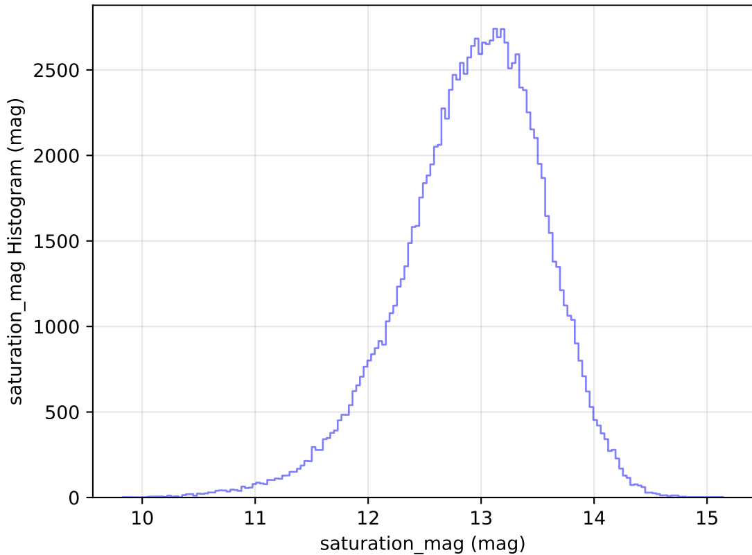
too_elab_r16_d3_griz_v3.4_10yrs WFD u band: saturation_mag Histogram
