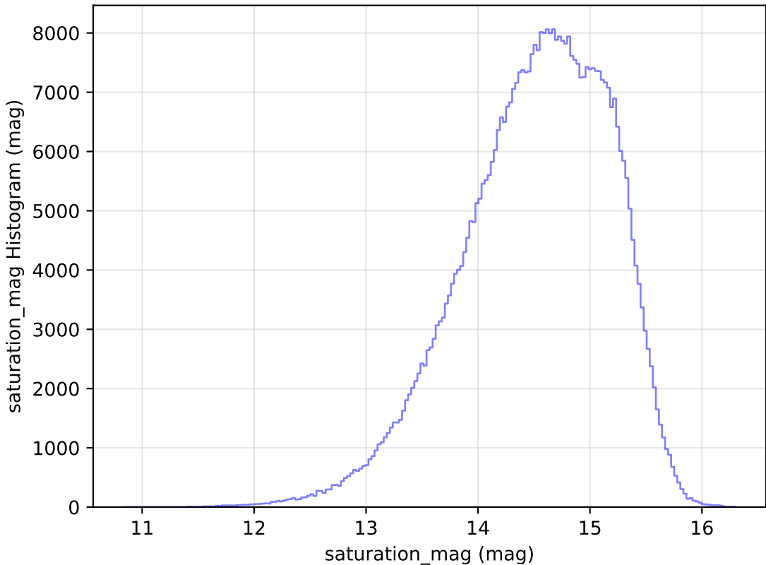
too_elab_r16_d3_griz_v3.4_10yrs WFD r band: saturation_mag Histogram
