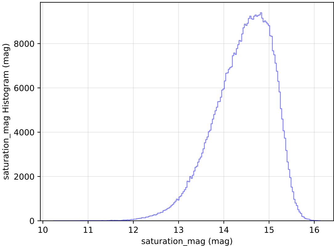
too_elab_r16_d3_griz_v3.4_10yrs WFD i band: saturation_mag Histogram
