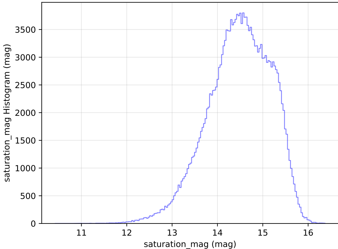
too_elab_r16_d3_griz_v3.4_10yrs WFD g band: saturation_mag Histogram
