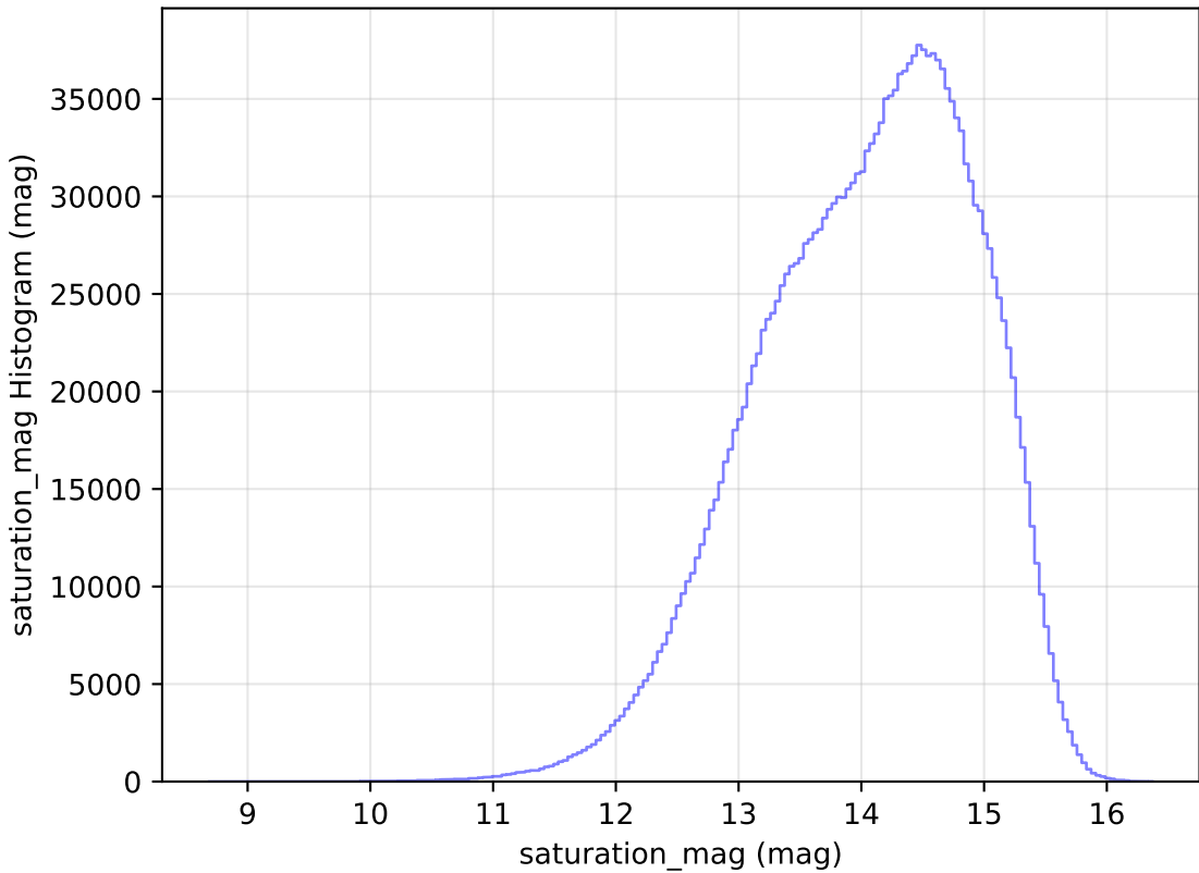
too_elab_r16_d3_griz_v3.4_10yrs WFD all bands: saturation_mag Histogram
