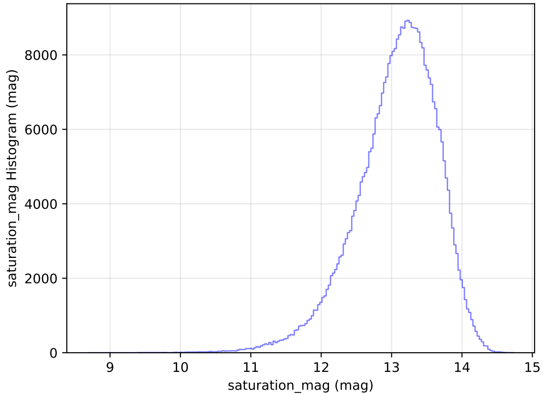
too_elab_r16_d3_griz_v3.4_10yrs All sky y band: saturation_mag Histogram
