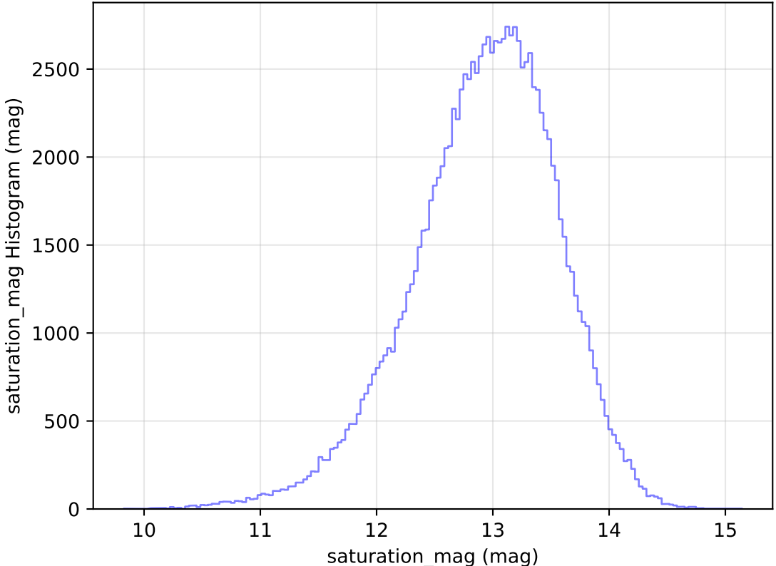
too_elab_r16_d3_griz_v3.4_10yrs All sky u band: saturation_mag Histogram
