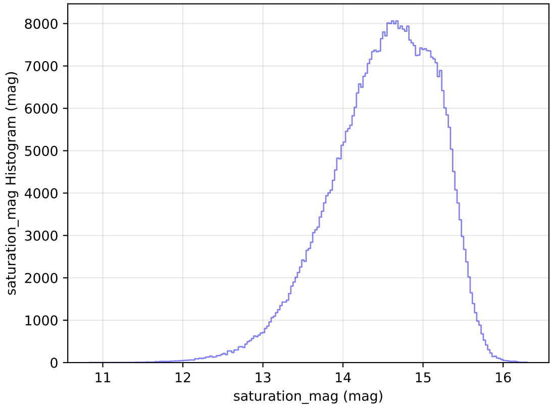
too_elab_r16_d3_griz_v3.4_10yrs All sky r band: saturation_mag Histogram
