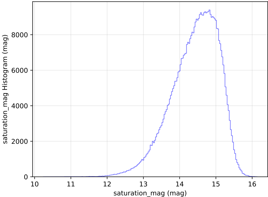
too_elab_r16_d3_griz_v3.4_10yrs All sky i band: saturation_mag Histogram
