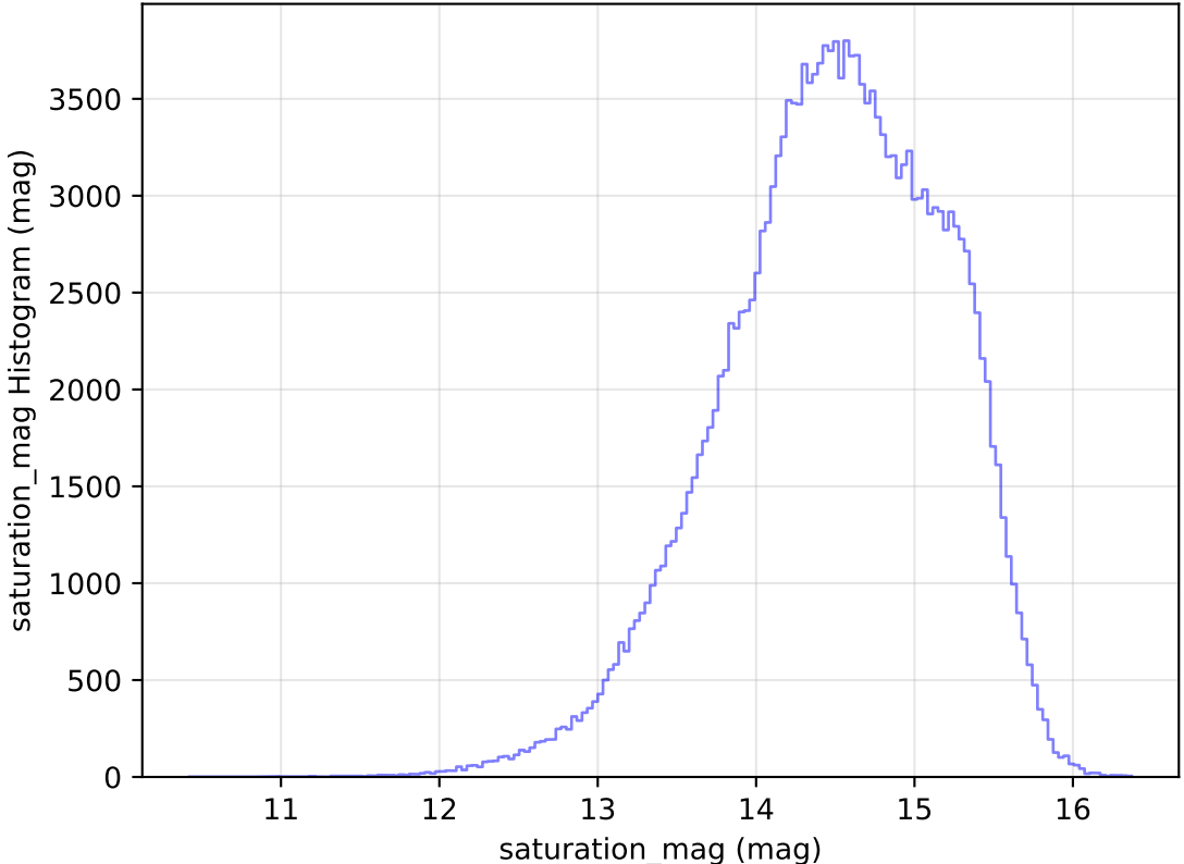
too_elab_r16_d3_griz_v3.4_10yrs All sky g band: saturation_mag Histogram
