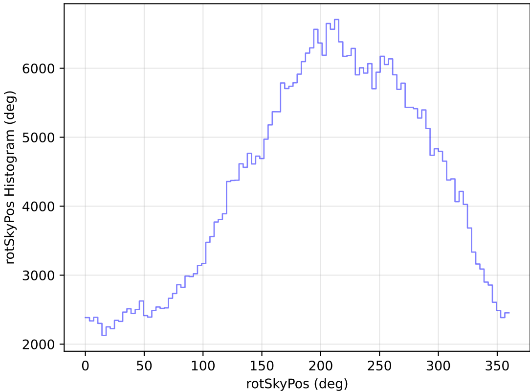
too_elab_r16_d3_griz_v3.4_10yrs WFD z band: rotSkyPos Histogram
