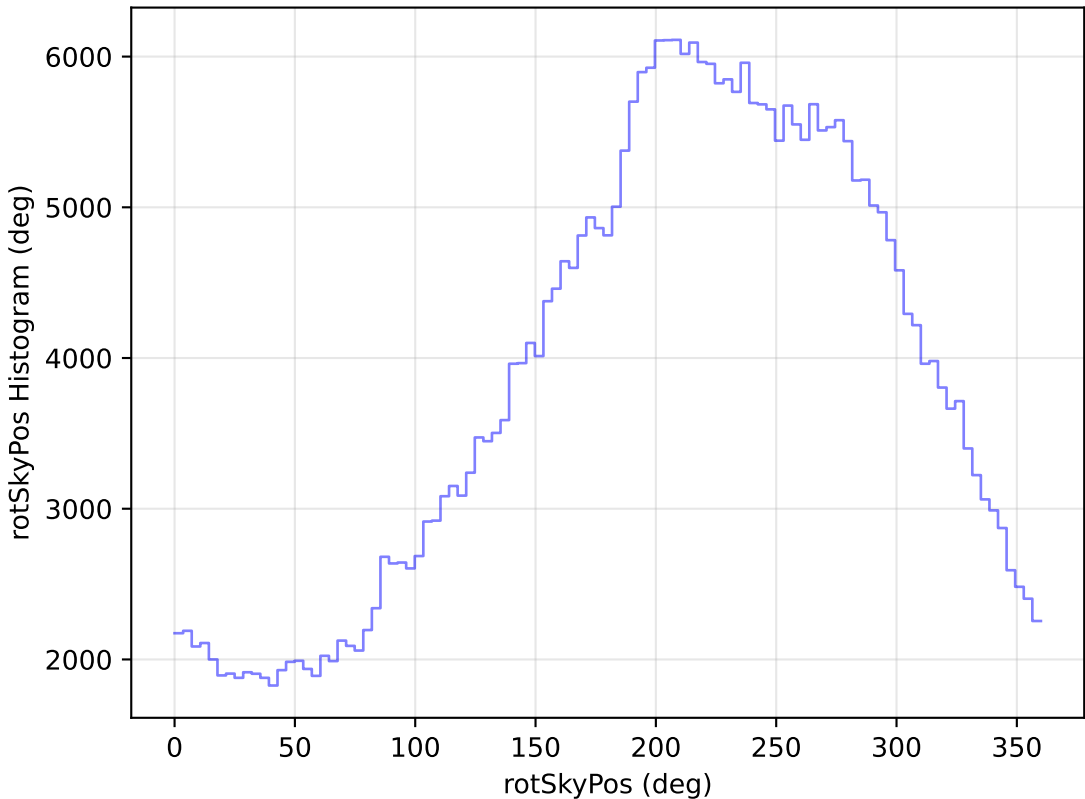
too_elab_r16_d3_griz_v3.4_10yrs WFD y band: rotSkyPos Histogram
