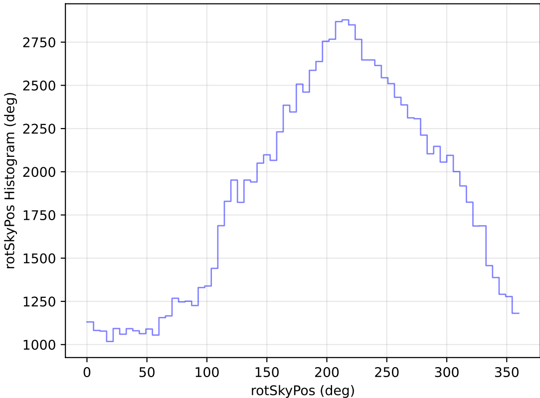
too_elab_r16_d3_griz_v3.4_10yrs WFD u band: rotSkyPos Histogram
