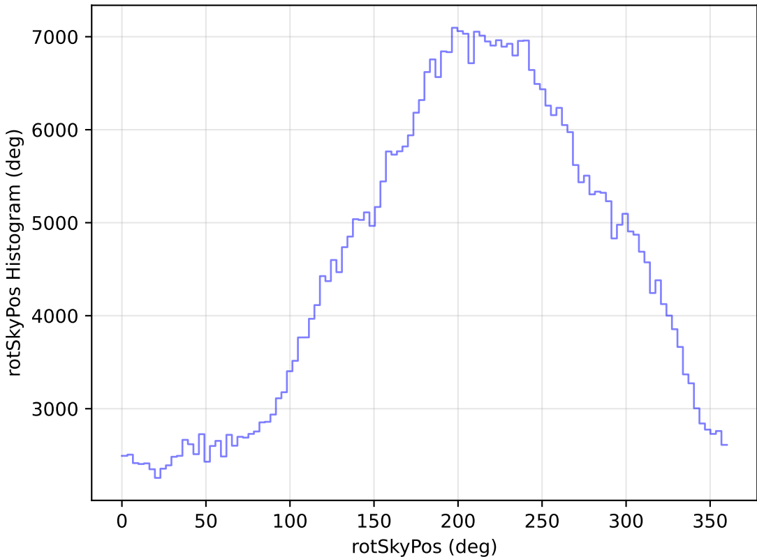
too_elab_r16_d3_griz_v3.4_10yrs WFD i band: rotSkyPos Histogram
