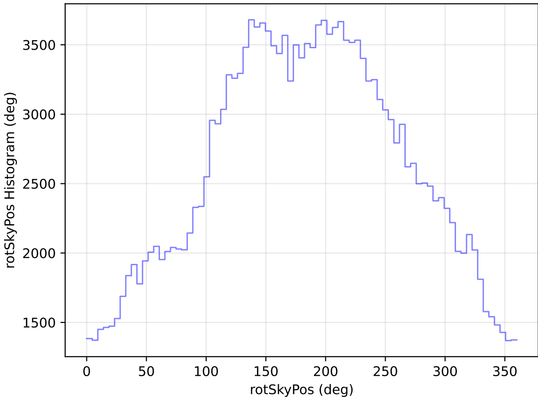
too_elab_r16_d3_griz_v3.4_10yrs WFD g band: rotSkyPos Histogram
