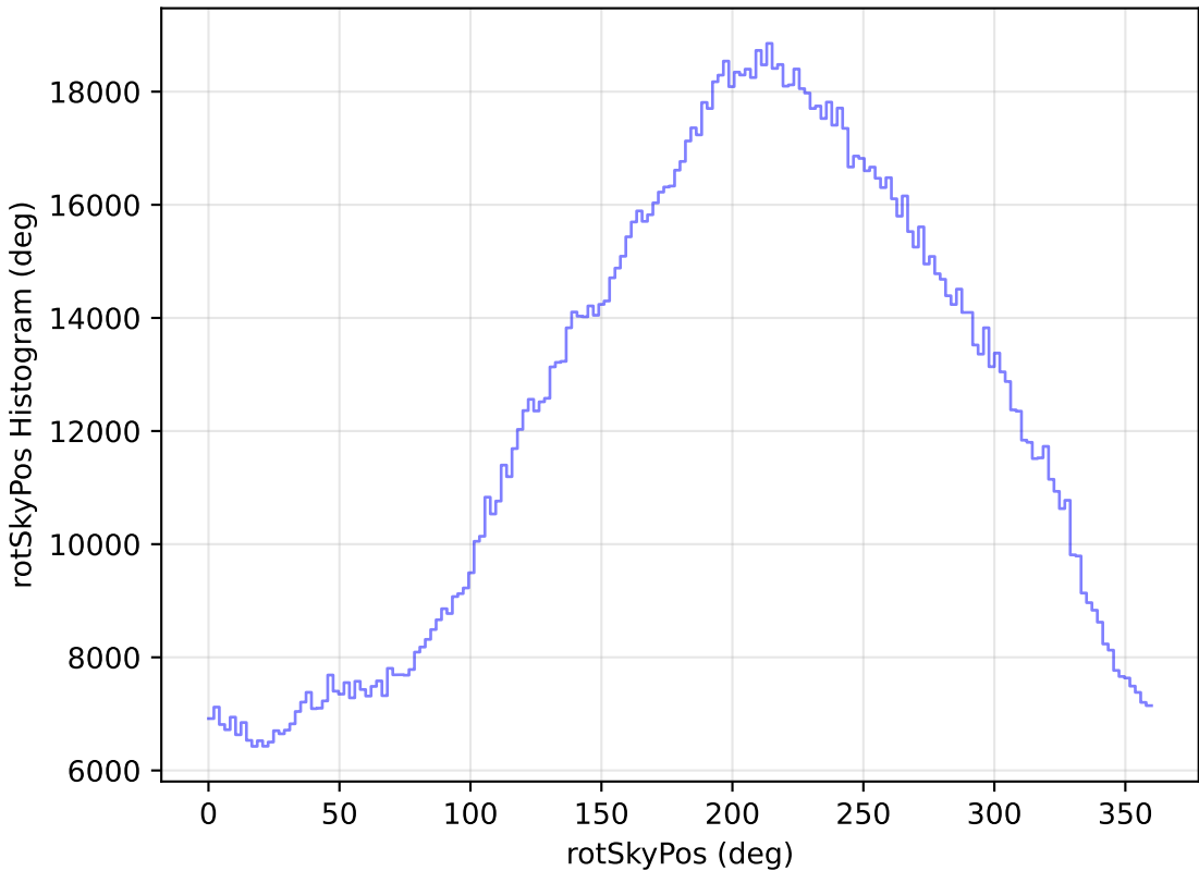
too_elab_r16_d3_griz_v3.4_10yrs WFD all bands: rotSkyPos Histogram
