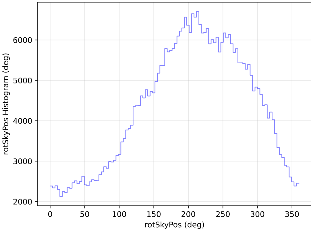
too_elab_r16_d3_griz_v3.4_10yrs All sky z band: rotSkyPos Histogram
