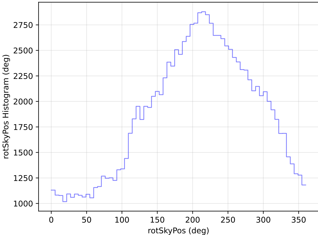
too_elab_r16_d3_griz_v3.4_10yrs All sky u band: rotSkyPos Histogram
