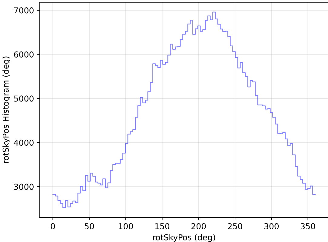
too_elab_r16_d3_griz_v3.4_10yrs All sky r band: rotSkyPos Histogram
