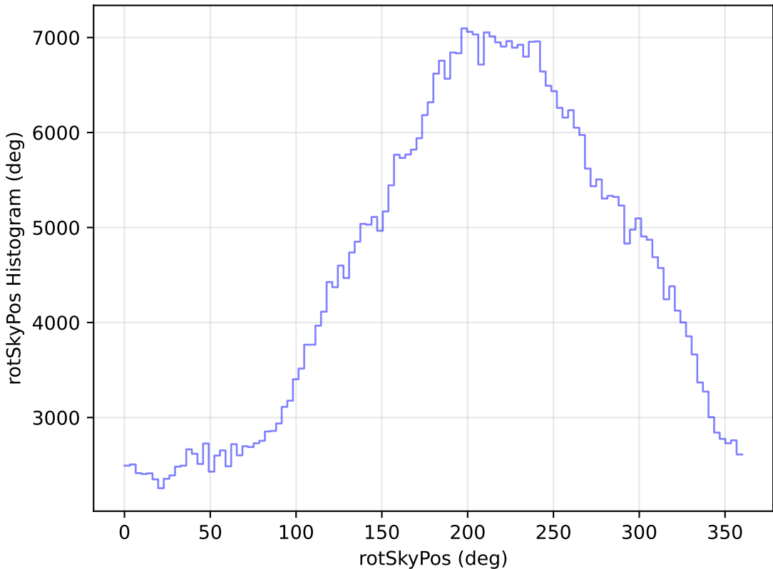
too_elab_r16_d3_griz_v3.4_10yrs All sky i band: rotSkyPos Histogram
