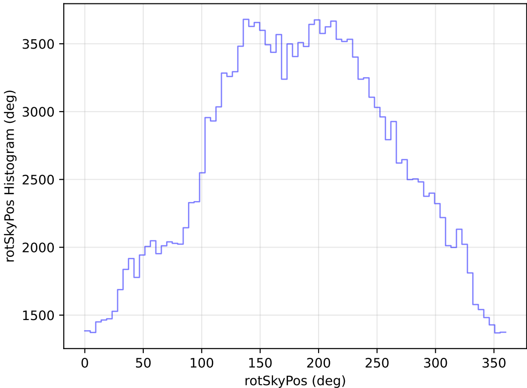
too_elab_r16_d3_griz_v3.4_10yrs All sky g band: rotSkyPos Histogram
