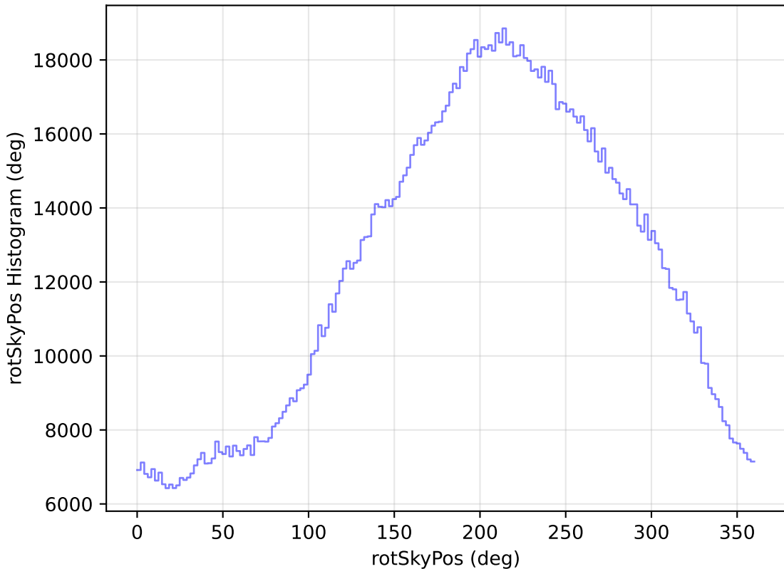
too_elab_r16_d3_griz_v3.4_10yrs All sky all bands: rotSkyPos Histogram
